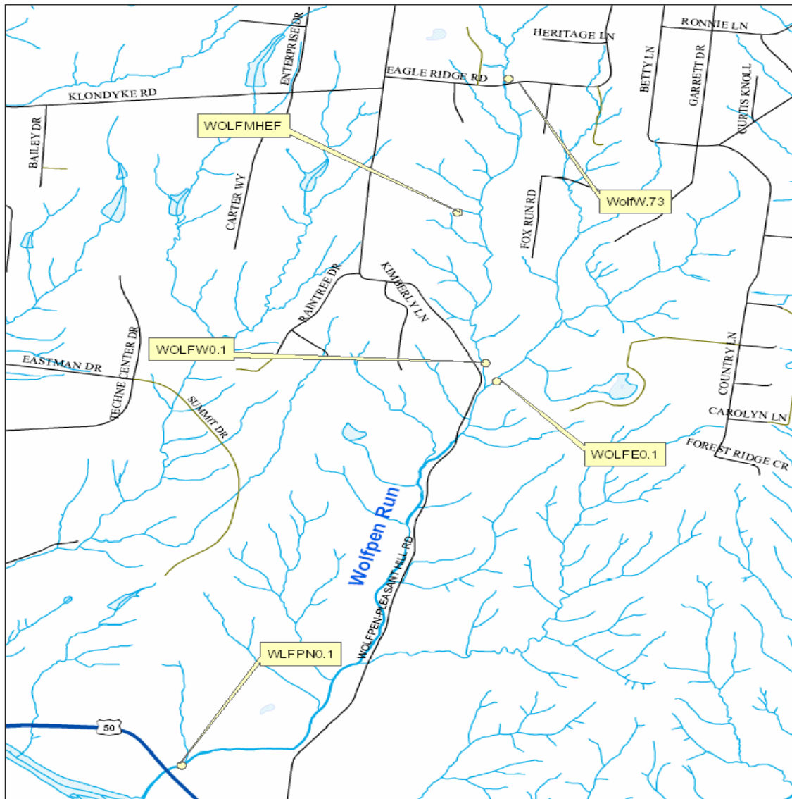
Figure 2. 2005 Dry Weather Survey – Wolfpen Run Sampling Locations.
