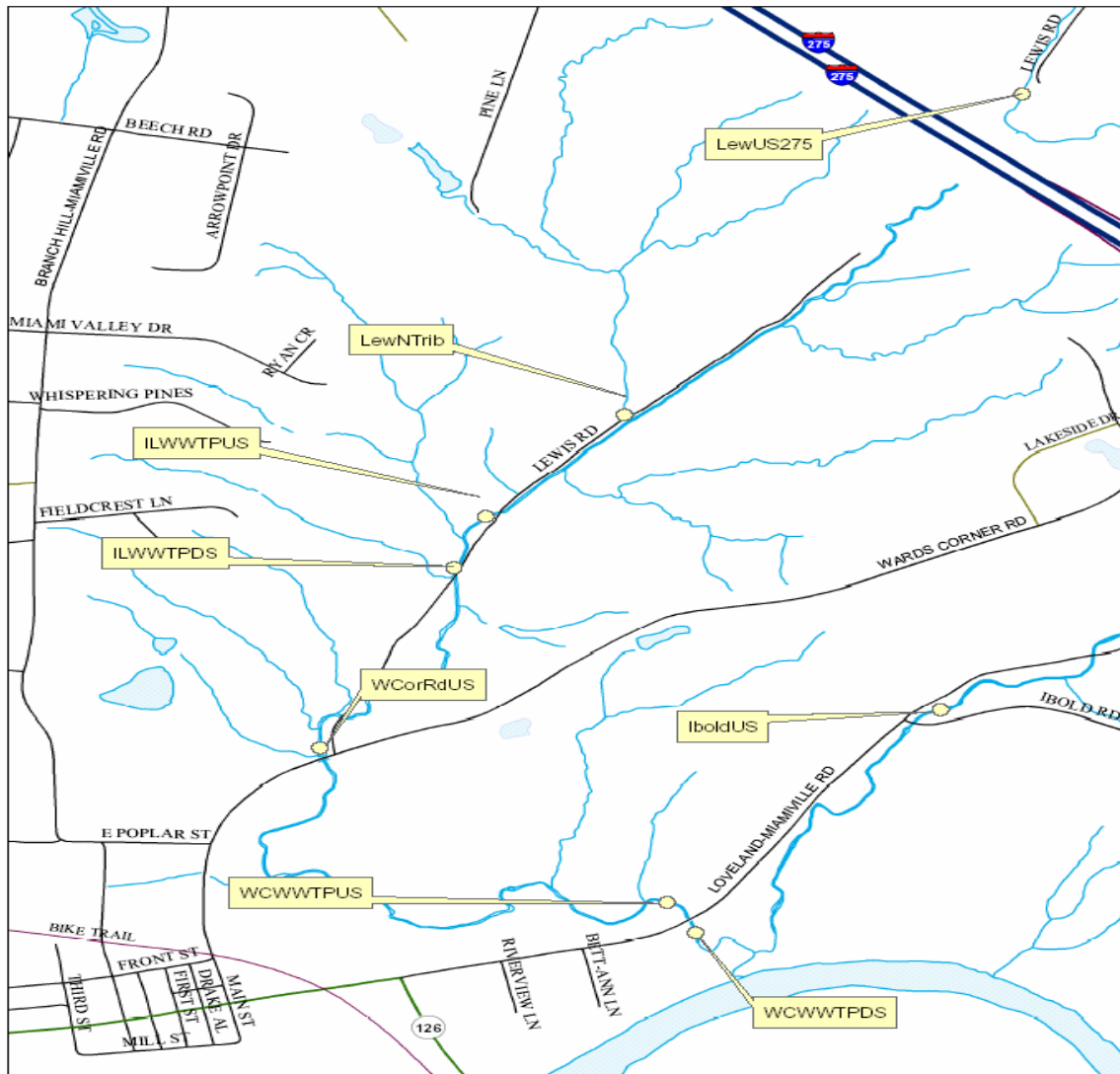
Figure 1. 2005 Dry Weather Survey - Miami Valley Sampling Locations.
